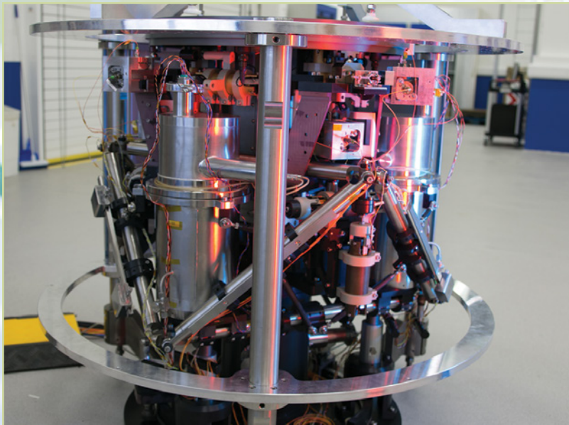
The micro-vibration test platform was designed to measure very low frequency related to very low force. (Image: National Physical Laboratory)
