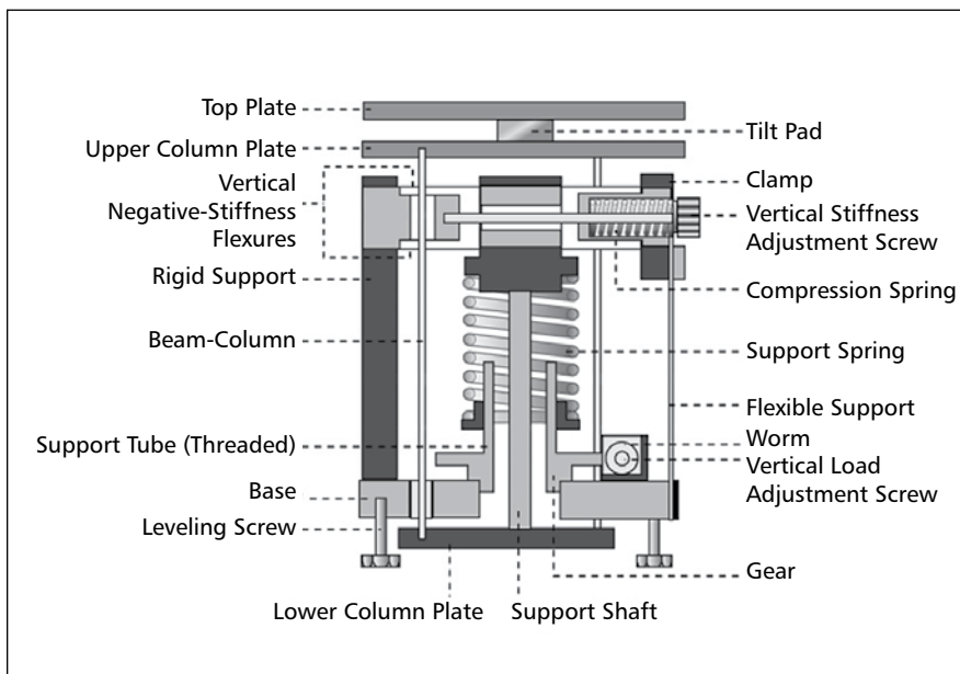
Schematic of a negative-stiffness isolator. (Image: National Physical Laboratory)
