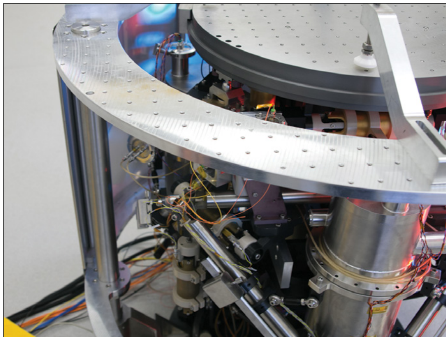
Upper measurement platform. (Image: National Physical Laboratory)
